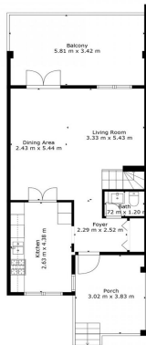
TOTAL: 103 m 2 FLOOR 1: 51 m 2 , FLOOR 2: 52 m 2 EXCLUDED AREAS: BALCONY: 23 m 2 , PORCH: 12 m 2 Floor Plan Created By Caviari App. Measurements Deemed Highly Reliable But Not Guaranteed.
